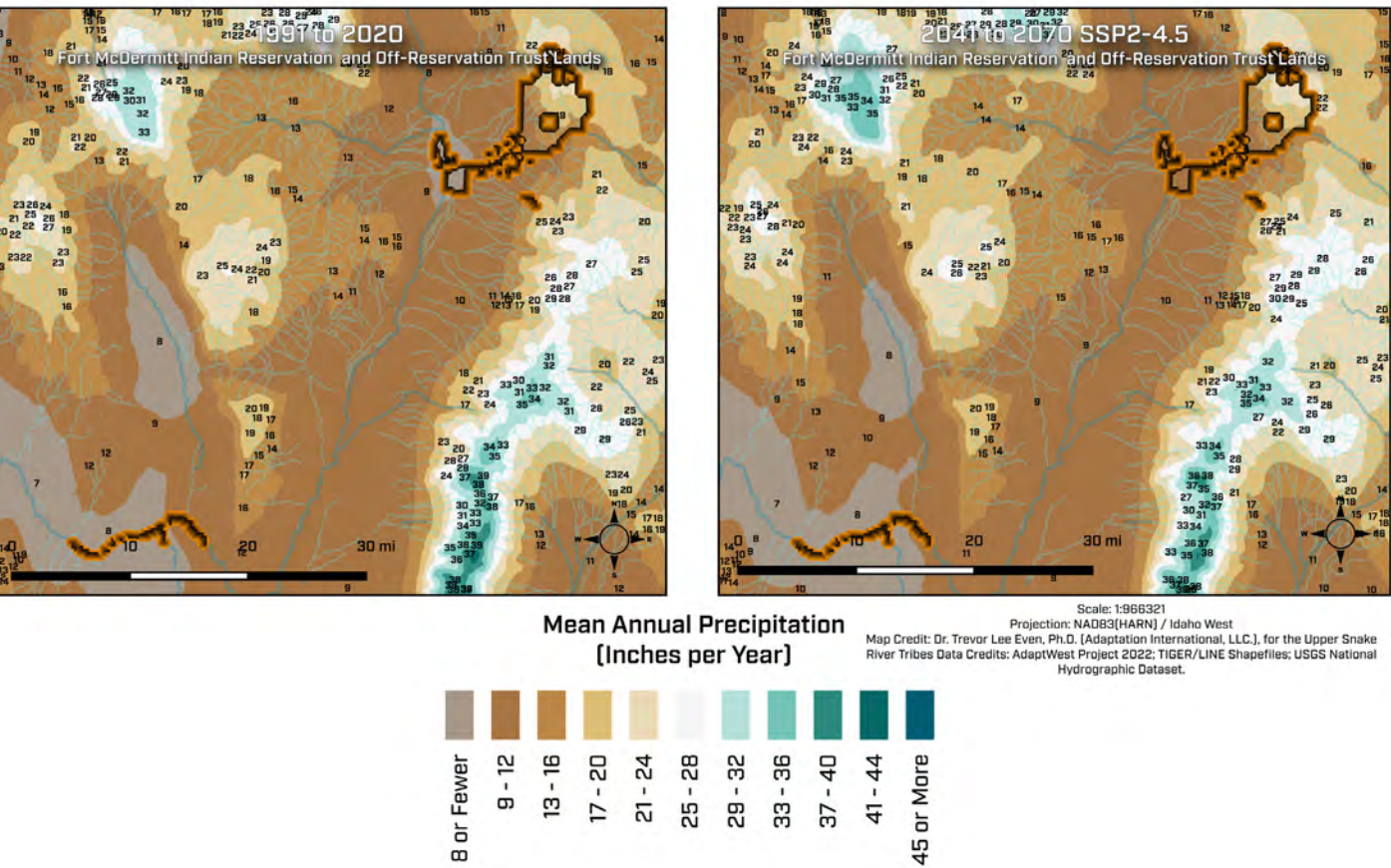
Fort McDermitt and Off-Reservation Trust Lands Mean Annual Precipitation, 1991-2020 and 2041-2070 projection.
