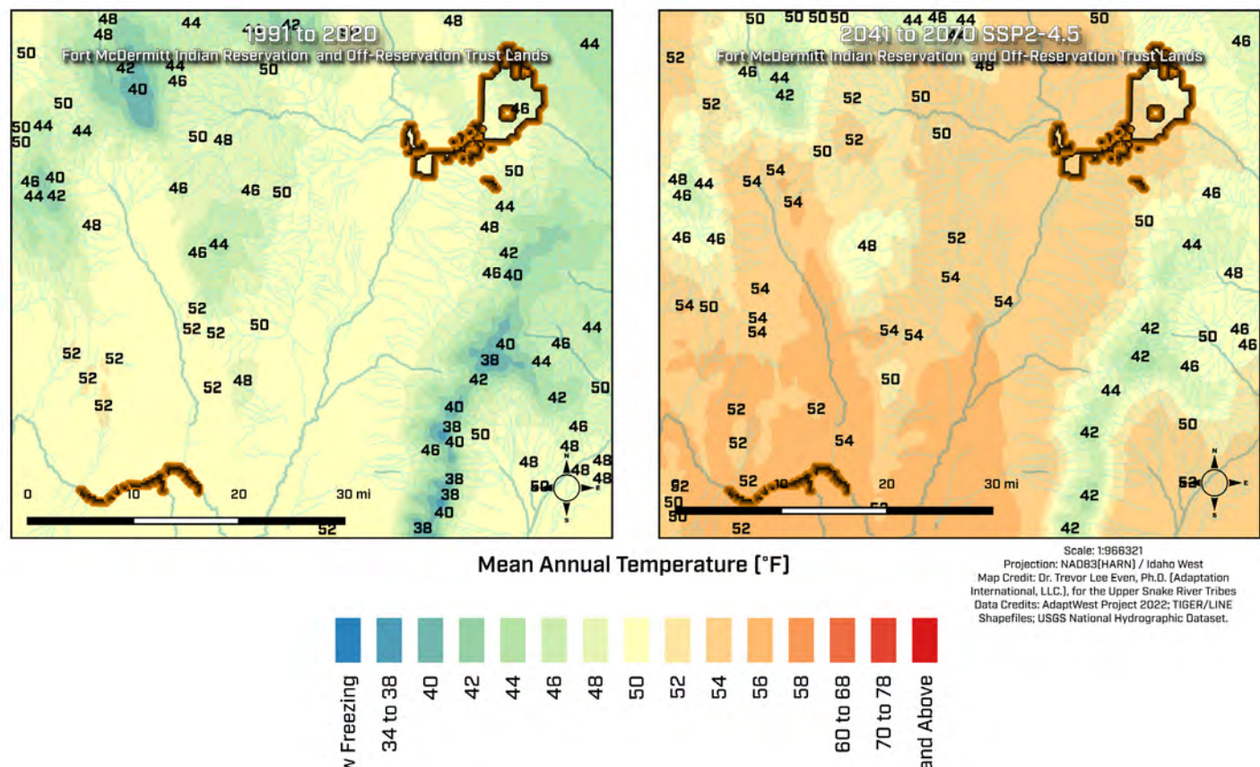
Fort McDermitt and Off-Reservation Trust Lands Mean Annual Temperatures, 1991-2020 and 2041-2070 projection.
